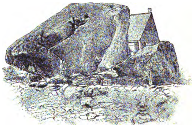
FIG. 60.—Vessel Rock, a glacial boulder in Gilsum, N. H. (C. H. Hitchcock.)
